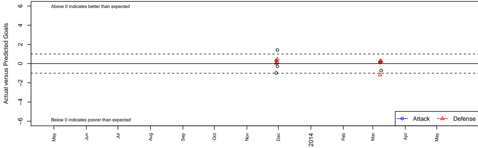
Players SC 00 Elite G99 Dots are actual minus expected GF (blue circles) and GA (red triangles). Blue line is smoothed change in attack strength. Red is smoothed change in defense strength.
